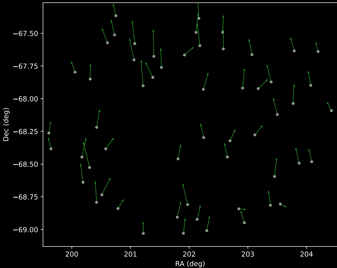
APOGEE DR17 Cluster 4 Proper Motion Vectors (n=56)
