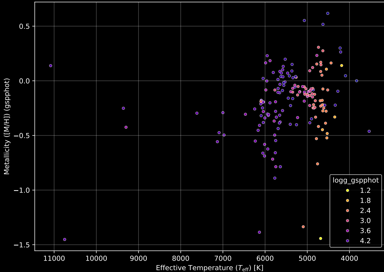
APOGEE DR17 Field: [279-25-O_TESS] Stellar Population Parameters (n= 170)
