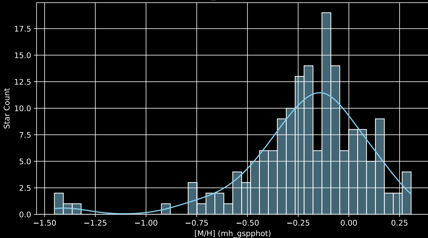
APOGEE DR17 Field: [279-25-O_TESS [M/H] (mh_gspphot) (n= 167)
