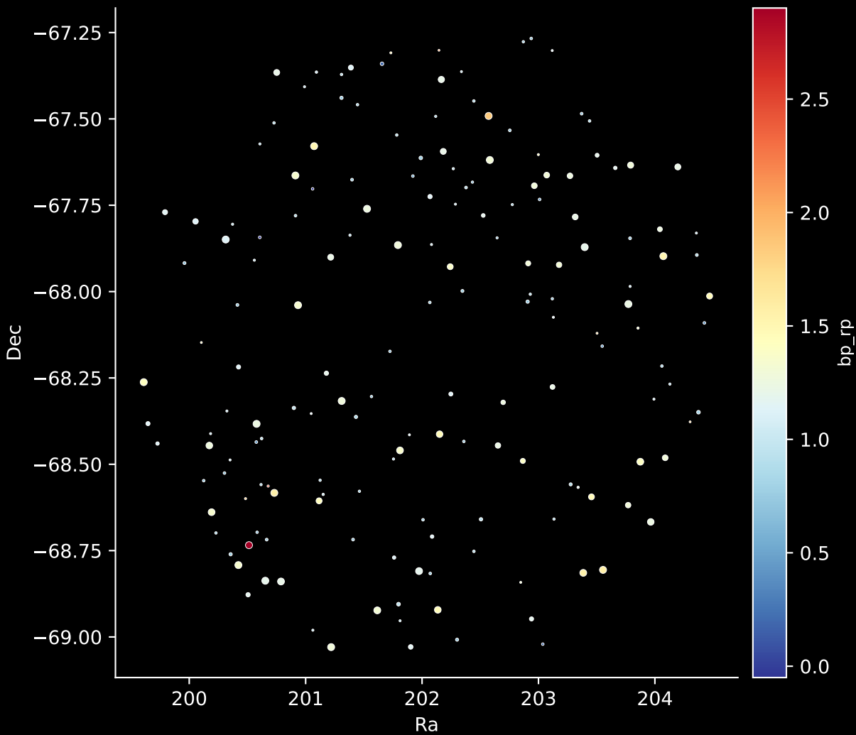
APOGEE DR17 Field: [279-25-O_TESS] Stars: 170
