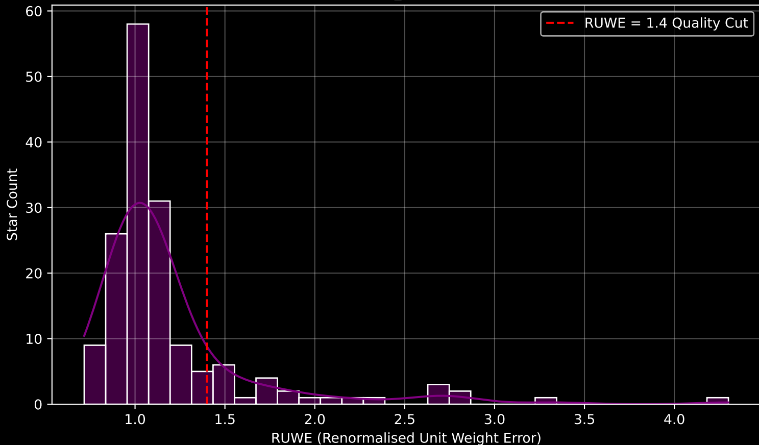
GAPOGEE DR17 Field [279-25-O_TESS] RUWE Distribution (n= 162)
