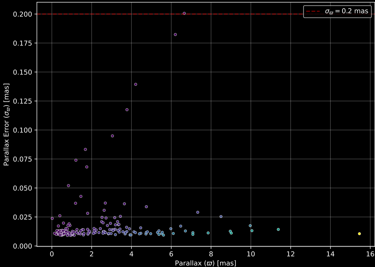
APOGEE DR17 Field: [279-25-O_TESS] Parallax Quality (n= 170)
