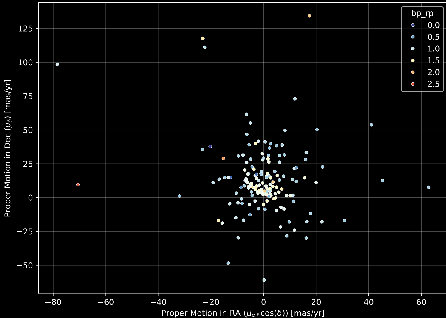
APOGEE DR17 Field: [279-25-O_TESS] Proper Motion Diagram (n= 170)
