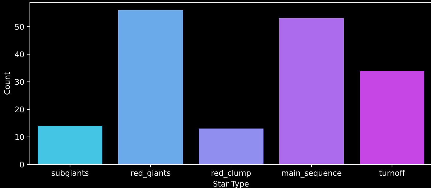
APOGEE DR17 Field: [279-25-O_TESS] Count plot of Star Type
